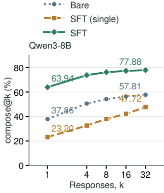
Figure 4: Effect of SFT label construction on Qwen3-8B \text{compose@k} .
