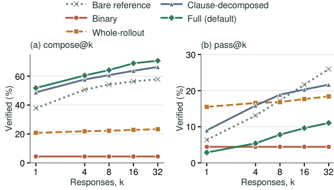
Figure 5: Qwen3-8B reward ablation from Base: (a) \text{compose@k} ; (b) \text{pass@k} . Vertical scales differ.
