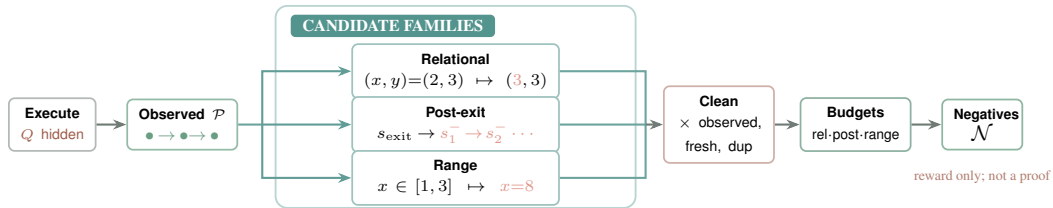
Figure 5: Construction of target-hidden negative traces. Concrete executions provide observed reachable states. Three transformations probe relational structure, behavior past a genuine exit, and sampled bounds. Conservative cleaning and per-family budgets produce \mathcal{N} , which is used only for RL reward computation and never exposes Q .
