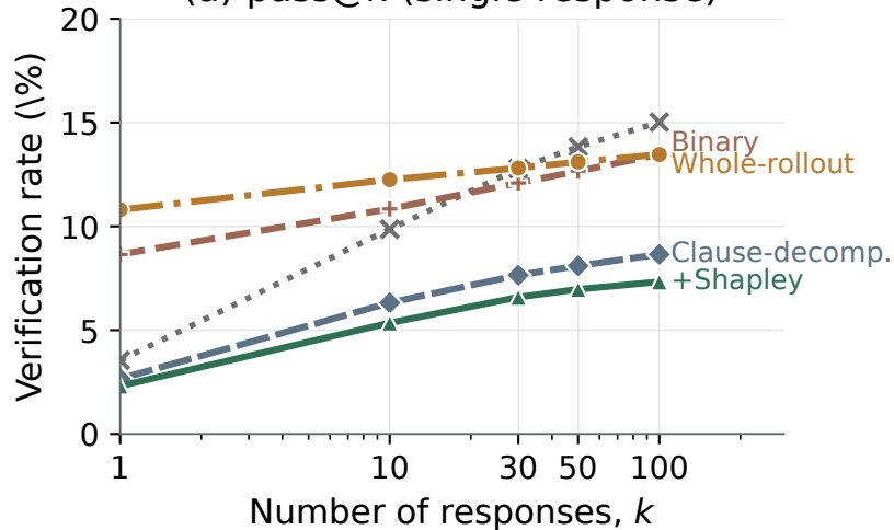
(a) pass@k (single response)
