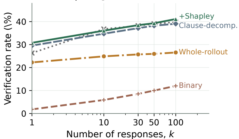
(b) compose@k (union + Houdini)
