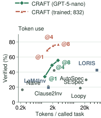
Figure 2: Verification versus tokens on each method’s full supported set. Direct GPT-5-nano results use 832 tasks, except Clause2Inv (316 Linear) and LaM4Inv (366 Linear+NLA). The dashed trained-CRAFT reference uses all 832. Squares mark the new LORIS and LaM4Inv adaptations.
