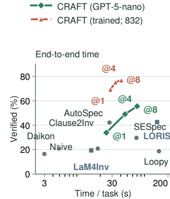
Figure 11: Verification versus time under native serving setups, using each method’s full supported set. Direct GPT-5-nano results use 832 tasks except Clause2Inv (316) and LaM4Inv (366); the dashed trained-CRAFT reference uses all 832. Daikon uses no model tokens.
