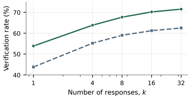
(b) compose@ k (composed responses)
