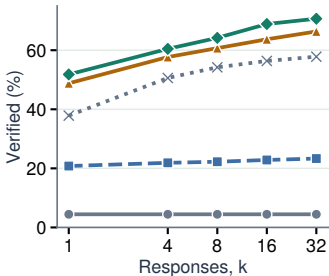
(a) compose@k
