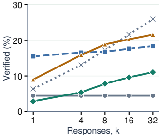
(b) pass@k
