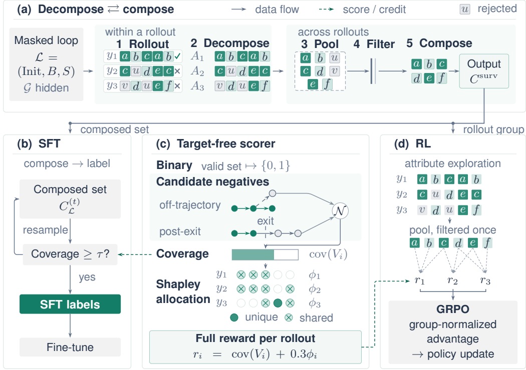
Figure 1: Decompose-compose is the organizing principle. (a) Pooling and joint filtering retain useful clauses from failed responses; letters track clause identity. (b) SFT distills coverage-accepted compositions. (c) Execution-derived candidate negatives supply coverage; Shapley allocation splits shared rejection credit. (d) Retained clauses credit their proposing rollouts for GRPO. The sampler inset shows off-trajectory perturbations and post-exit body continuations. The hidden target \mathcal{G} is restored only for final verification.
