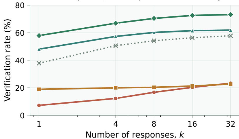
(a) compose@ k : compositional coverage
