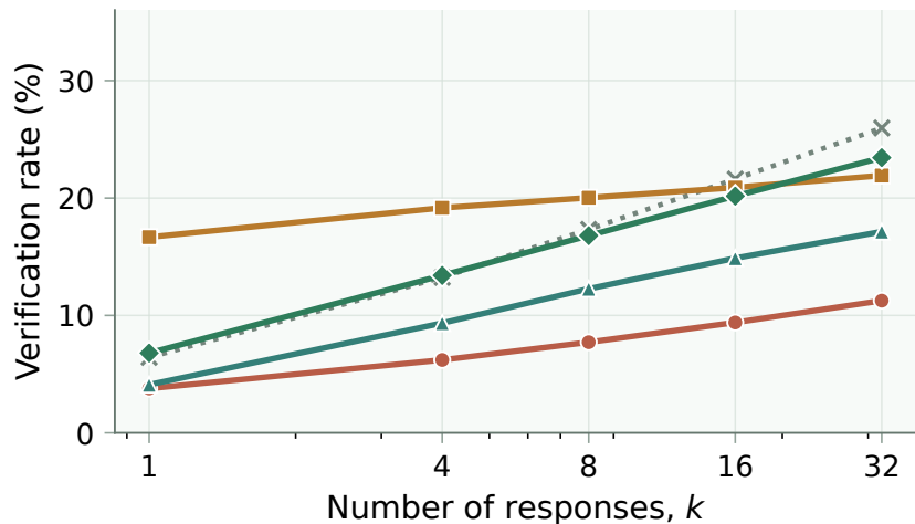
(b) pass@ k : response-level coverage
