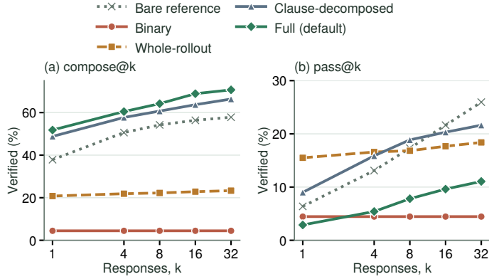
Figure 5: Qwen3-8B reward ablation from Base: (a) compose@k; (b) pass@k. Vertical scales differ.
