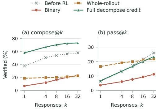
Figure 4: Qwen3-8B reward ablations from the Bare initialization. Whole-response credit reduces composition; clause credit recovers it. The matched SFT-initialized controls, where Binary collapses the strong SFT composition curve, are in Table 18.
