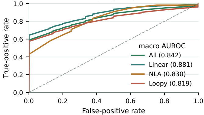
(a) Within-program prediction
