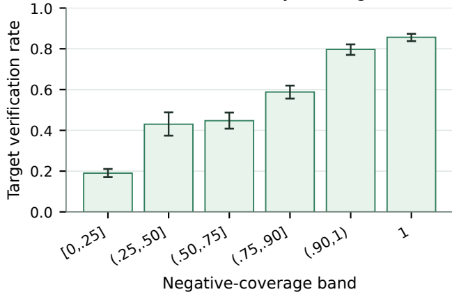
(b) Verification by coverage
