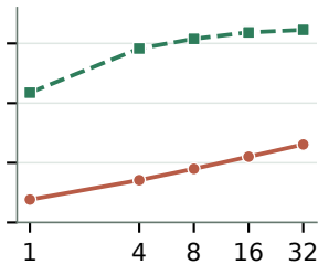
(c) Qwen3-14B
