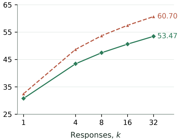
(b) pass@ k
