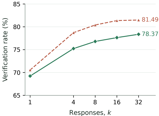
(a) compose@ k
