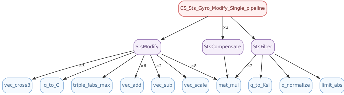
Fig. 10. Call graph of the single-star-sensor filter-update pipeline. Edge labels show call multiplicity; unlabeled edges are \times 1 .
