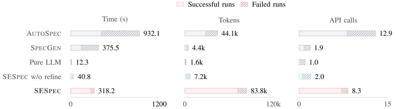
Fig. 4. Mean cost per attempted program on all 400 gpt-5.4-mini cases. Each bar stacks valid-run (solid) and failed-run (hatched) contributions, each divided by 400.
