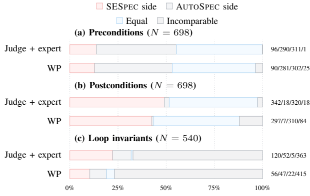
Fig. 3. Dimension-wise relations for AUTOSPEC versus SESPEC over identical data sets. A directional segment means a more permissive accepted domain for preconditions and a logically stronger predicate for postconditions or invariants. “Judge + expert” is the corrected judge result; WP checks the same implications. Right-hand counts follow the legend order.
