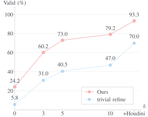
Fig. 12. Cumulative Valid rate on gpt-5.4-mini over 400 cases as the refinement budget k increases, for the full SESPEC pipeline ( Ours ) versus a trivial refine baseline.
