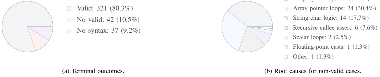
Fig. 6. Failure outcome and root-cause summary for the gpt-5.4-mini SESPEC-400 rerun.
