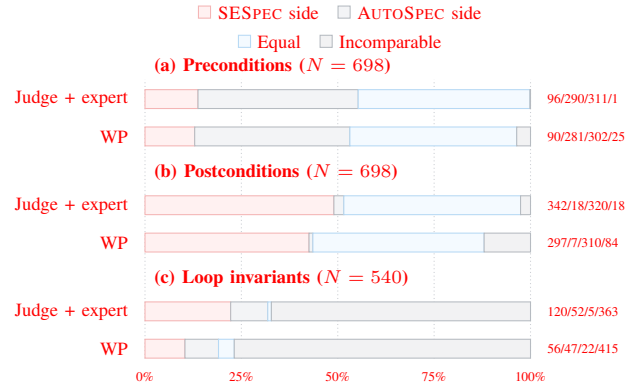
Fig. 4. Dimension-wise relations for AUTOSPEC versus SESPEC over identical data sets. A directional segment means a more permissive accepted domain for preconditions and a logically stronger predicate for postconditions or invariants. “Judge + expert” is the corrected judge result; WP checks the same implications. Right-hand counts follow the legend order.
