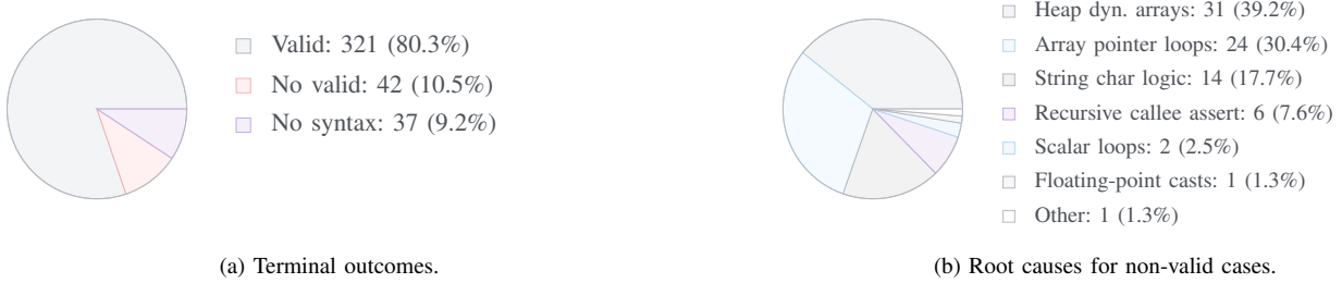
Fig. 6. Failure outcome and root-cause summary for the gpt-5.4-mini SESPEC-400 rerun.
