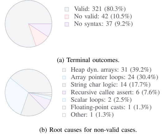
Fig. 5. Failure outcome and root-cause summary for the gpt-5.4-mini SESPEC-400 rerun.
