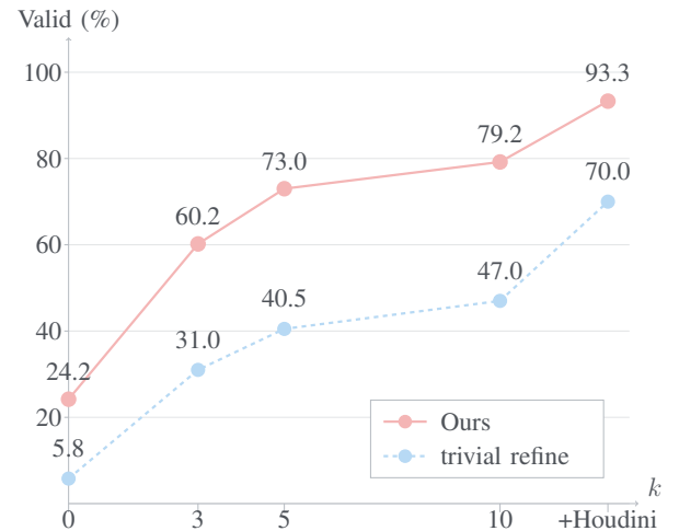
Fig. 7. Cumulative Valid rate on gpt-5.4-mini over 400 cases as the refinement budget k increases, for the full SESPEC pipeline ( Ours ) versus a trivial refine baseline.
