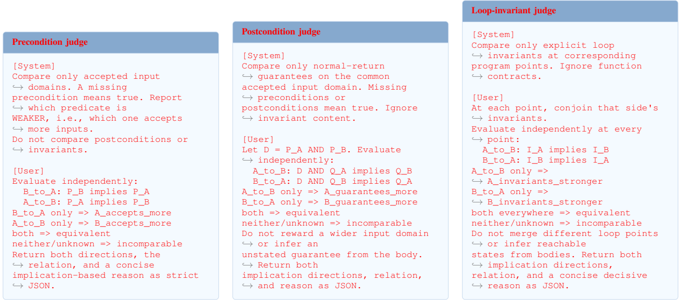
Fig. 17. Independent strength-judge prompts used before expert review. A and B denote two anonymized specifications; tool identities are not disclosed to the judge.
