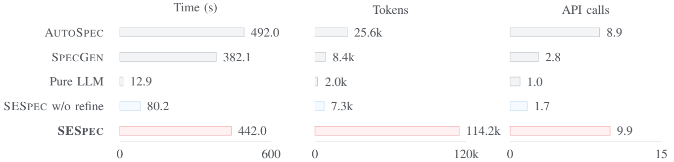
Fig. 5. Average cost per valid run on SESPEC-400 .
