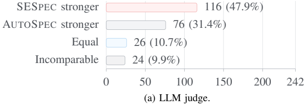
Fig. 4. Pairwise strength distribution on the 242 both-valid gpt-5.4-mini pairs against AUTOSPEC, comparing the LLM judge with a Frama-C/WP implication check.
