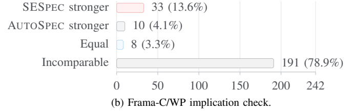
Fig. 4. Pairwise strength distribution on the 242 both-valid gpt-5.4-mini pairs against AUTOSPEC, comparing the LLM judge with a Frama-C/WP implication check.
