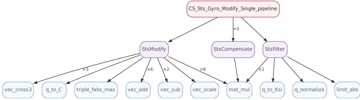
Fig. 13. Call graph of the single-star-sensor filter-update pipeline. Edge labels show call multiplicity; unlabeled edges are \times 1 .
