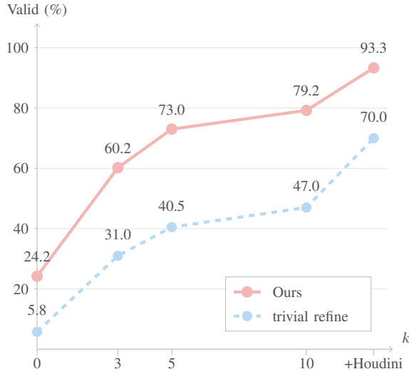
Fig. 7. Cumulative Valid rate on gpt-5.4-mini over 400 cases as the refinement budget k increases, for the full SESPEC pipeline ( Ours ) versus a trivial refine baseline.
