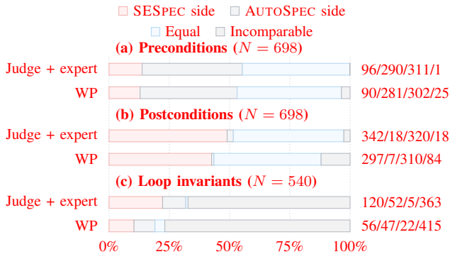
Fig. 3. Dimension-wise relations for AUTOSPEC versus SESPEC over identical data sets. A directional segment means a more permissive accepted domain for preconditions and a logically stronger predicate for postconditions or invariants. “Judge + expert” is the corrected judge result; WP checks the same implications. Right-hand counts follow the legend order.
