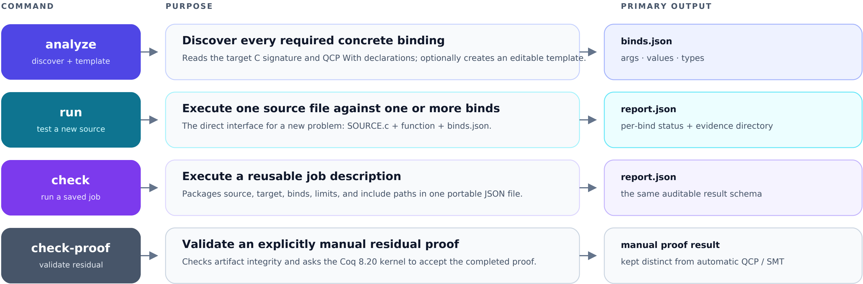
Figure 2. The public command-line surface; all execution and classification paths are deterministic.
