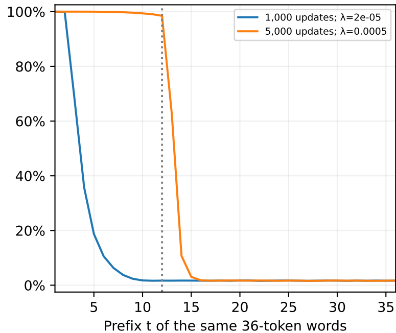
A(t): Only state t correct
