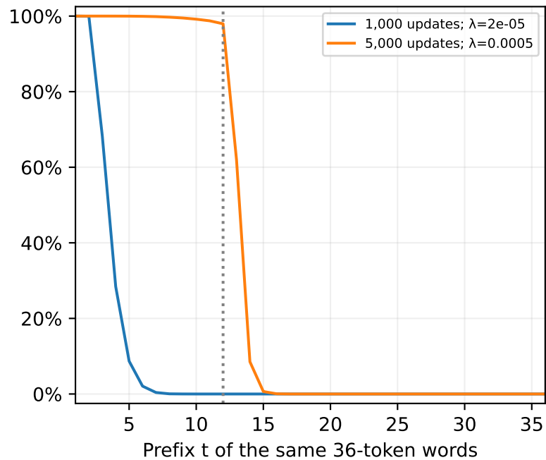
E(t): All states through t correct
