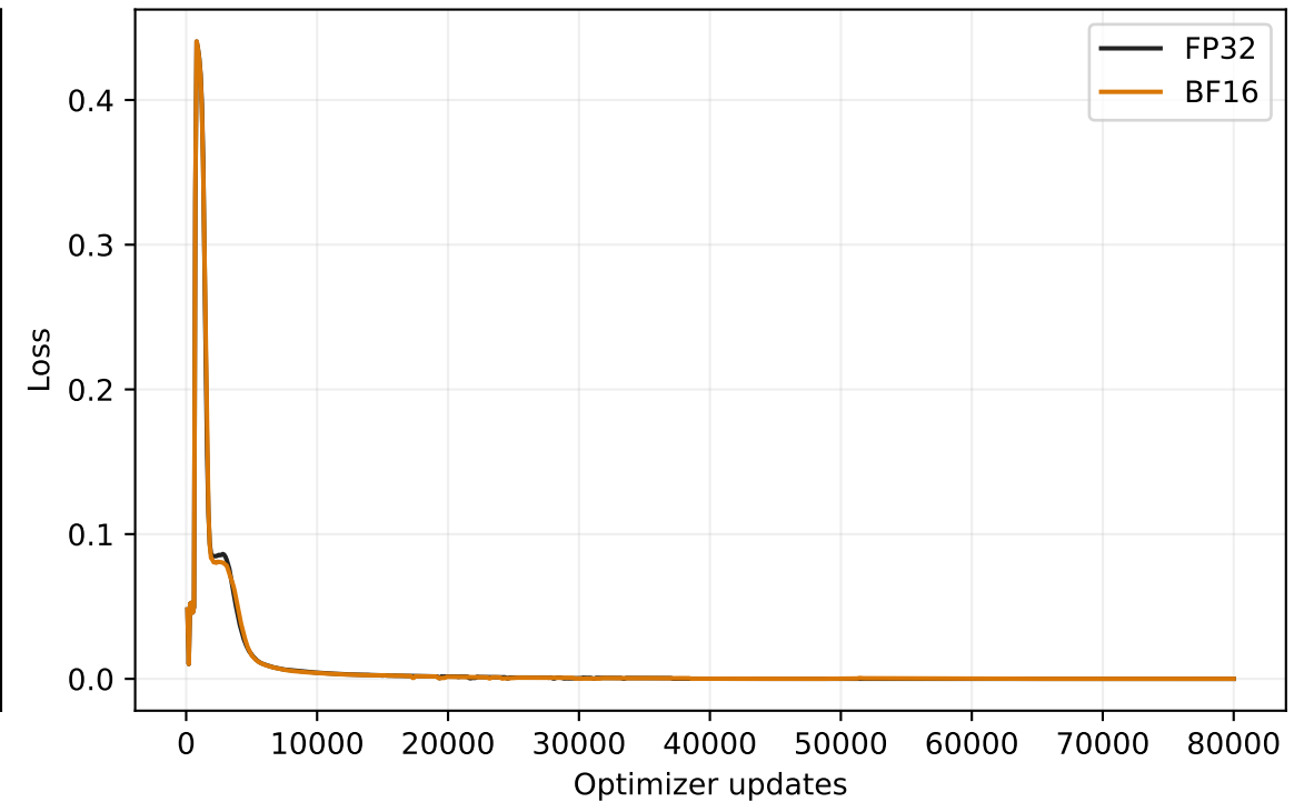
NextLat loss
