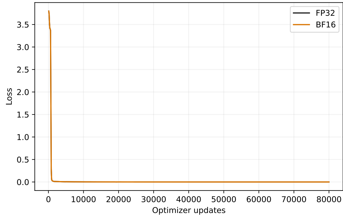
State cross-entropy
