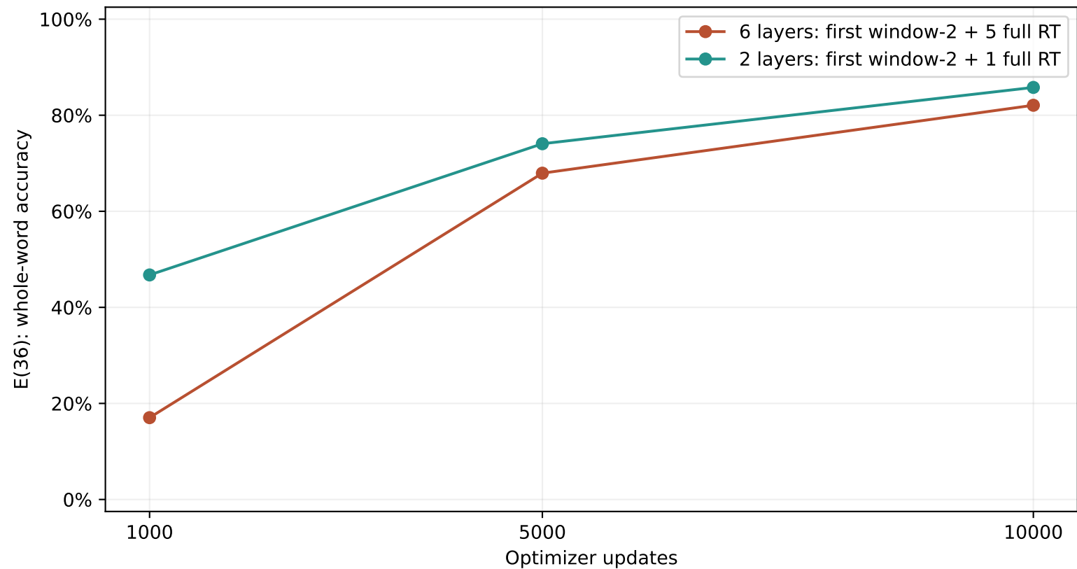
Length-36 whole-word accuracy at matched retained checkpoints
