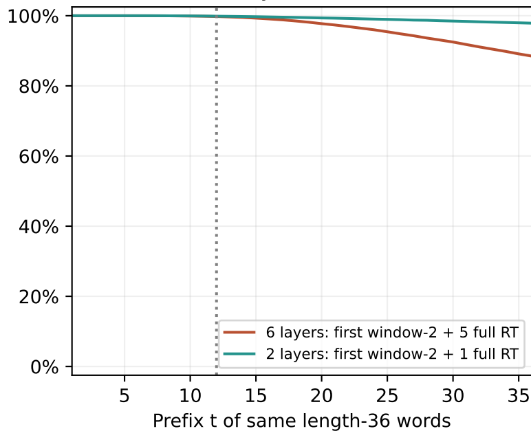
A(t): Only state t correct
