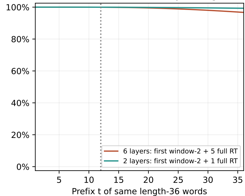
M(t): Mean token accuracy through t
