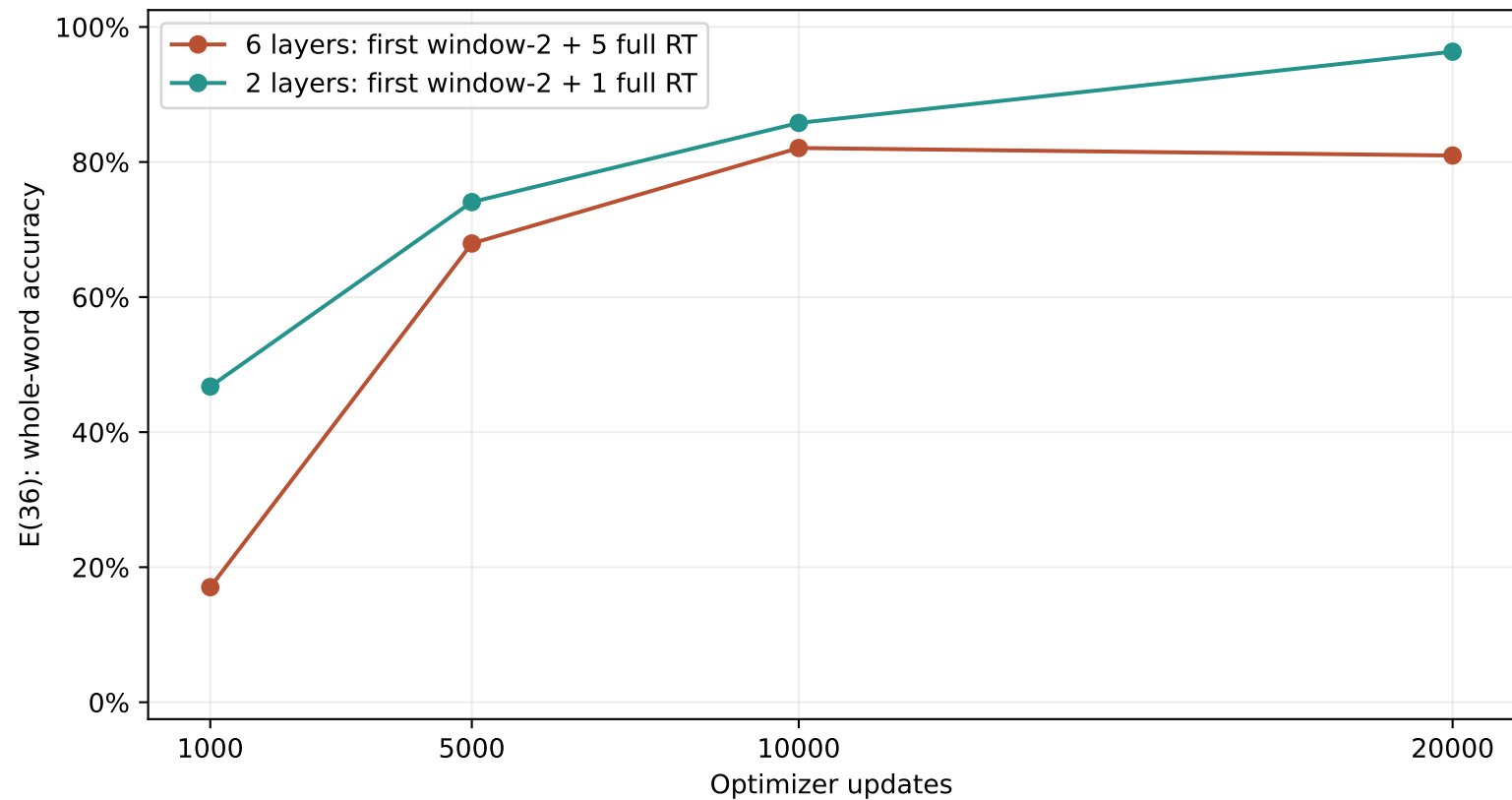
Matched length-36 whole-word accuracy · 15k excluded from primary comparison
