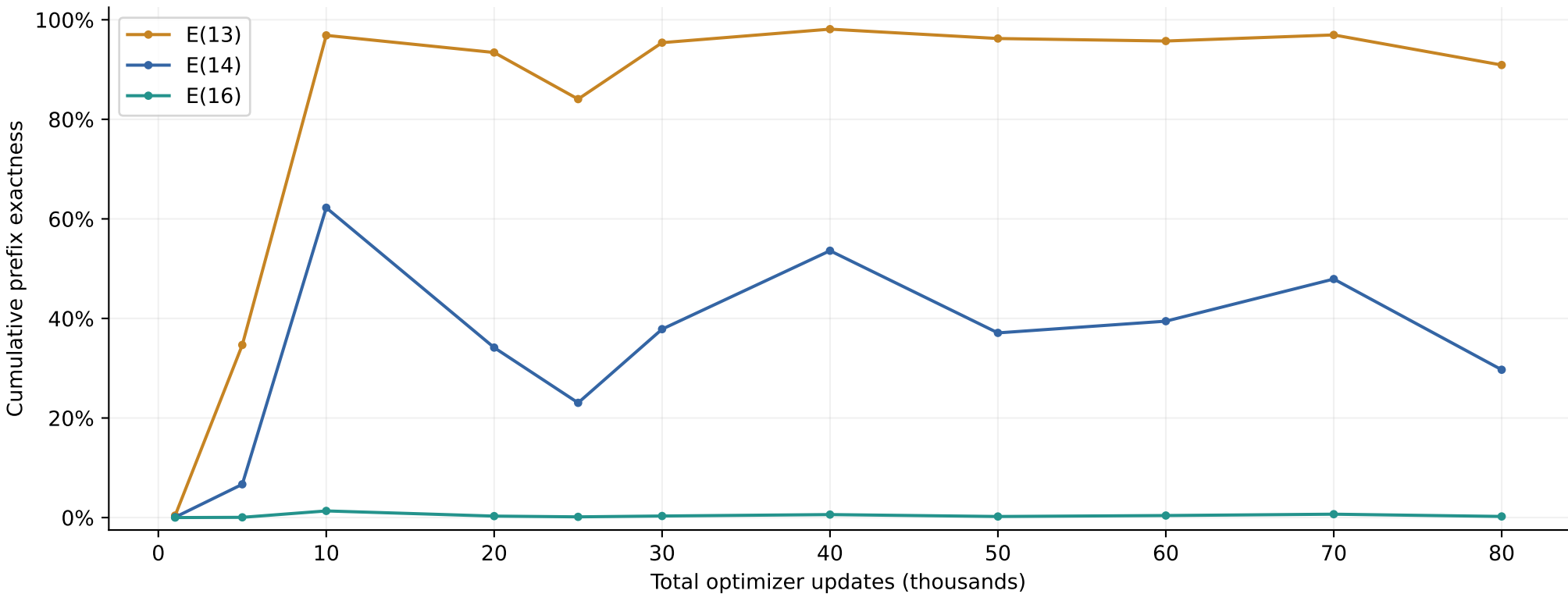
RT + NextLat · fixed development prefixes versus training budget
