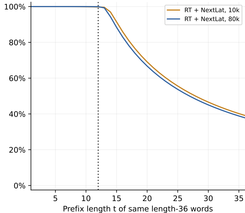
M: mean token accuracy through t
