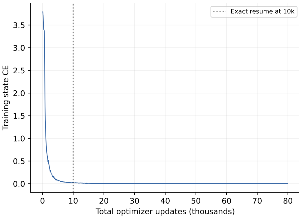
Original RT + NextLat · complete pilot + continuation · nonoverlapping 100-update means
