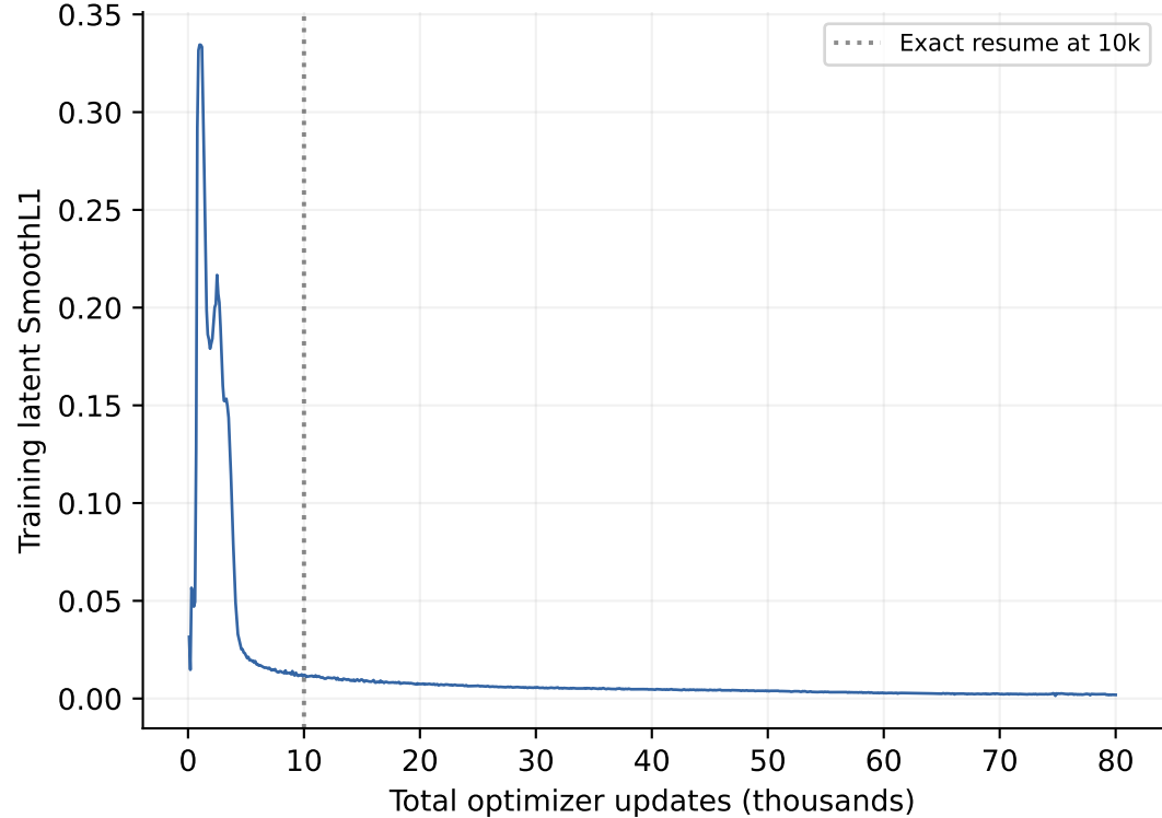
Original RT + NextLat · complete pilot + continuation · nonoverlapping 100-update means
