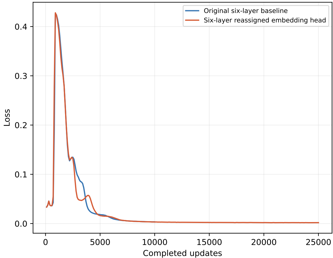
NextLat SmoothL1, 100-update means
