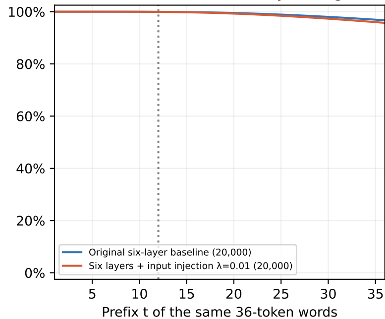
M(t): Mean token accuracy through t
