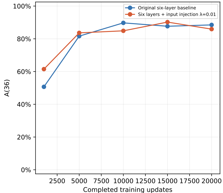
Full 102,400-word development evaluations at each arm's retained checkpoints
