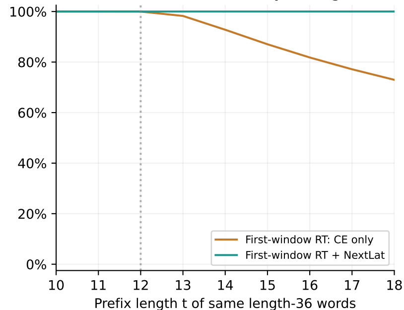
M: mean token accuracy through t
