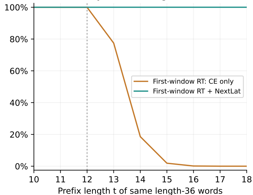
E: every state through t correct
