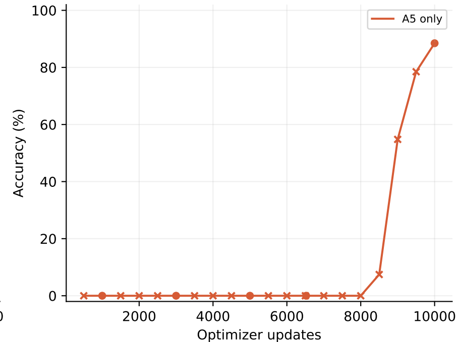
A5 length 36: Whole-word exactness
