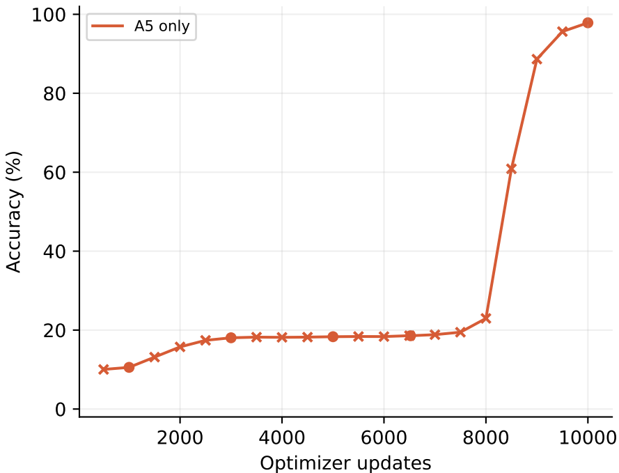
A5 length 36: Mean token accuracy
