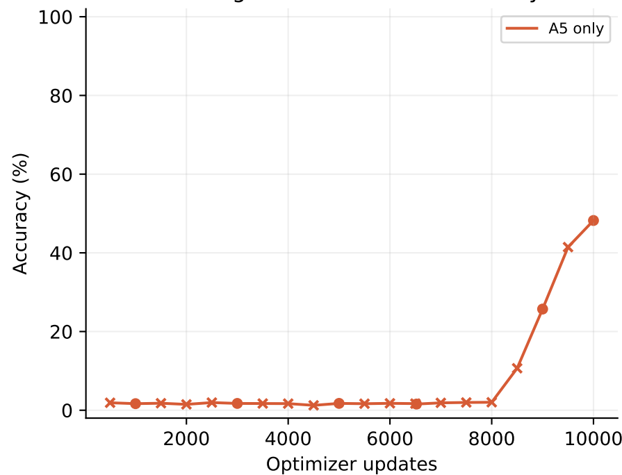
A5 length 36: Final-state accuracy
