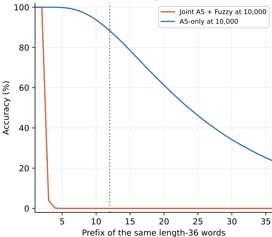
E(t): cumulative prefix exactness
