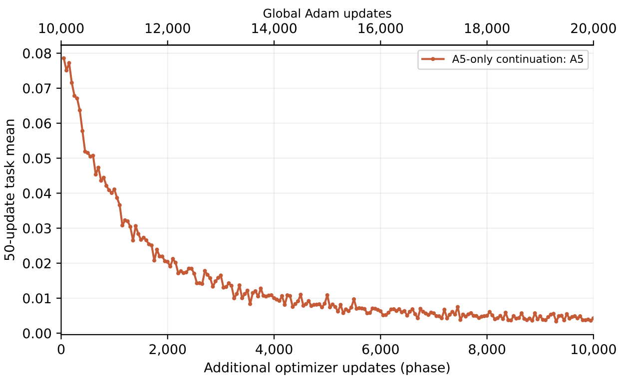
Unweighted task CE
