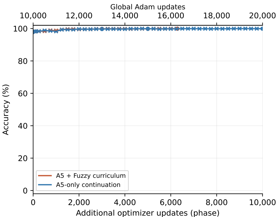
A5 length 36: Mean token accuracy
