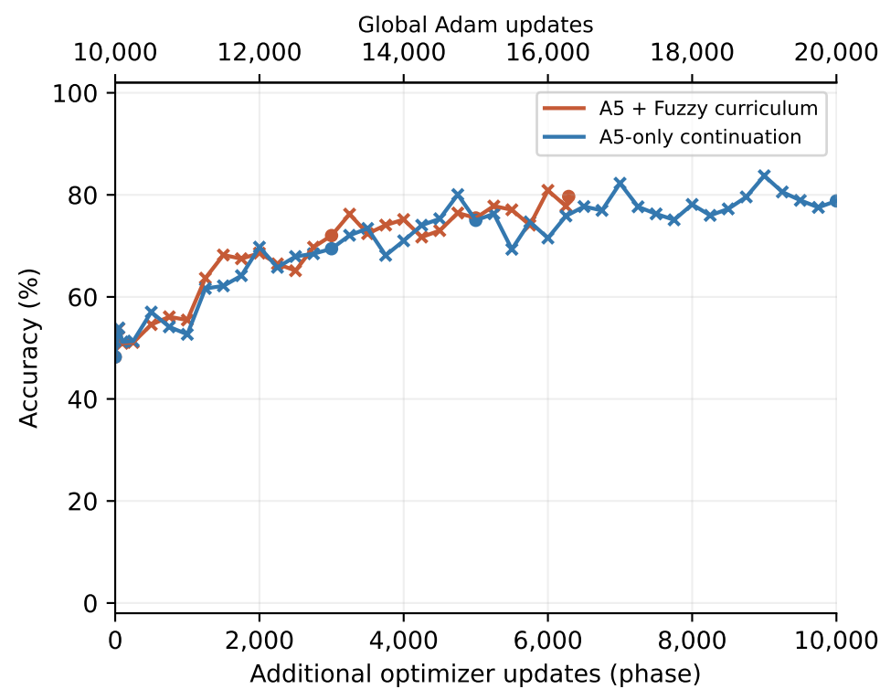
A5 length 36: Final-state accuracy
