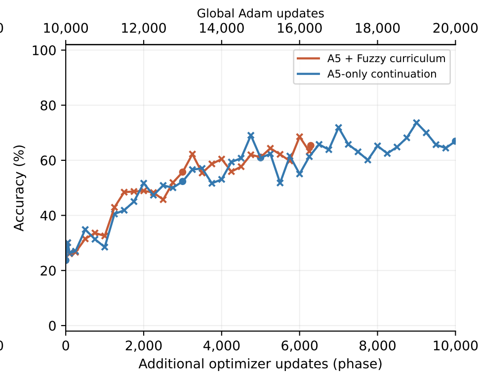
A5 length 36: Whole-word exactness
