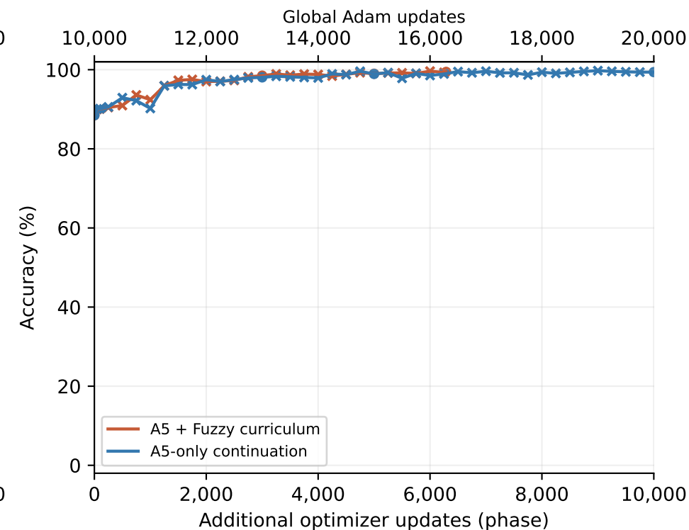
A5 length 36: Whole-word exactness
