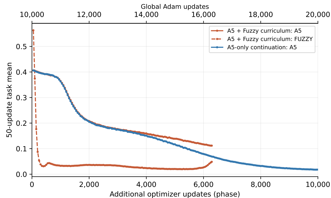
Unweighted task NextLat SmoothL1
