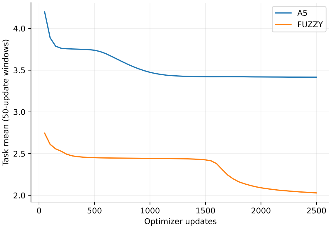
Task losses averaged separately; Fuzzy CE is dense, A5 CE scores every state Per-task training CE
