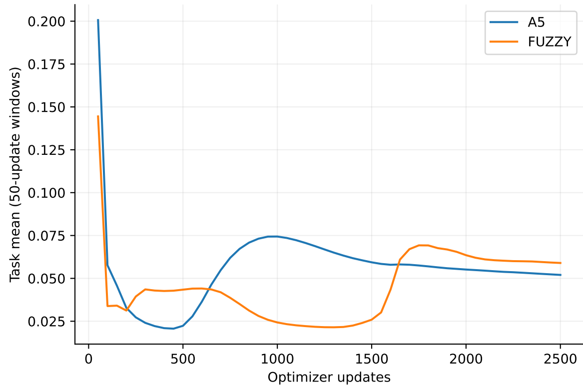
Task losses averaged separately; Fuzzy CE is dense, A5 CE scores every state Per-task training CE
