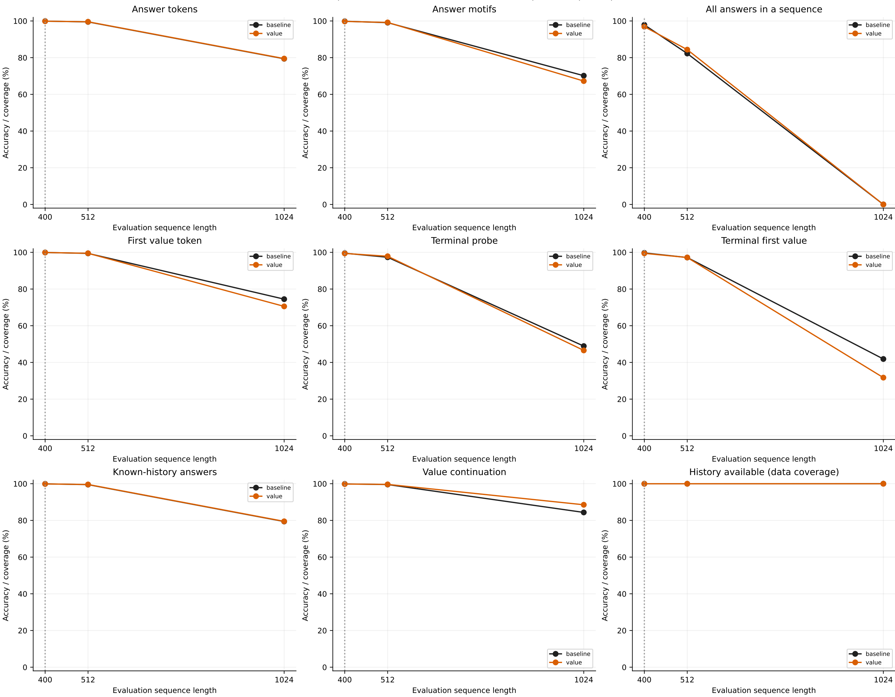
Fuzzy length generalization at fixed 15k checkpoints — trained T400, no new training T400 saved endpoint; T512/T1024 new shared 1,280-example development pools
