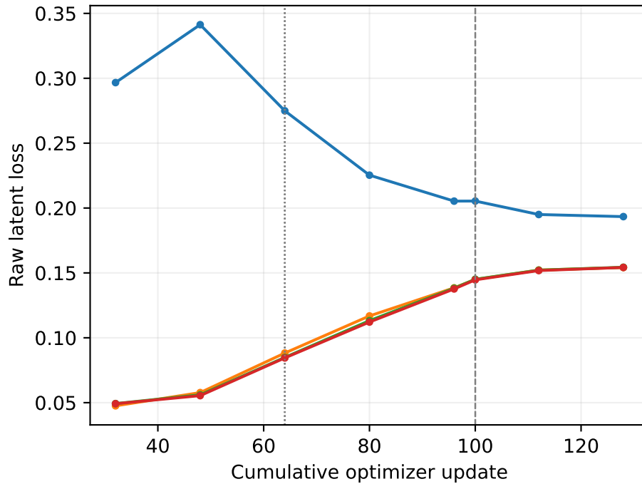
Reduced-KL NFR: common FP32/no-jitter development panel Continued from 64; unchanged KL0.1, latent1, K4, RT0/15; warmup ends at 100
