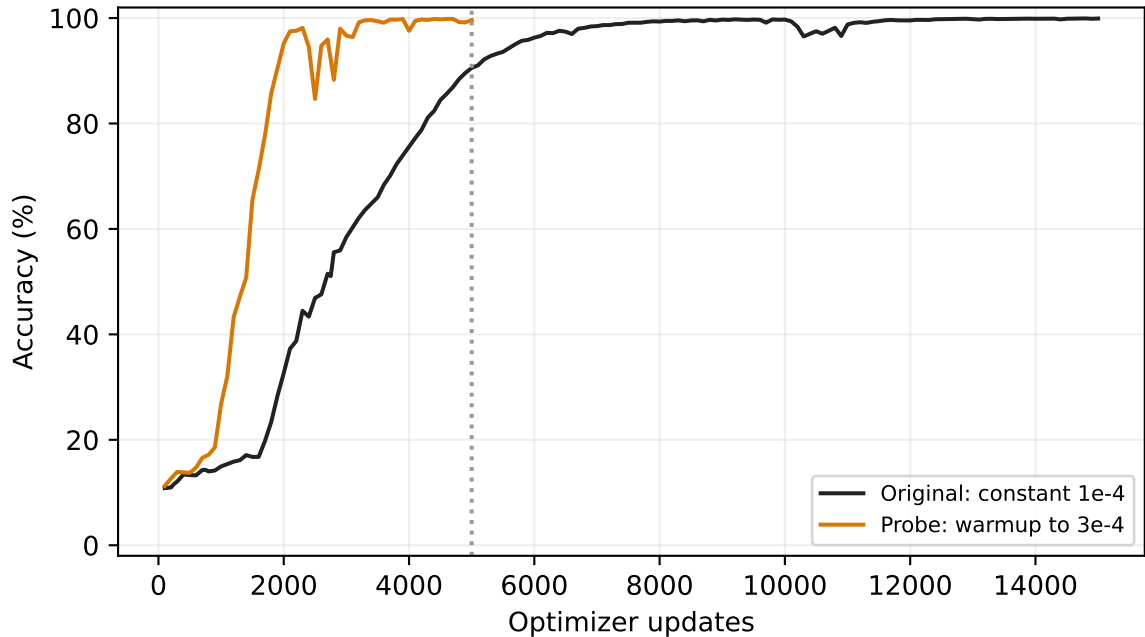
Fuzzy answer accuracy
