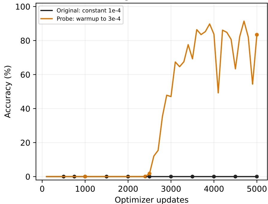
Fuzzy first value
