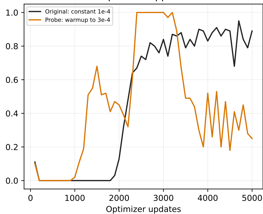
Fraction updates clipped at norm1
