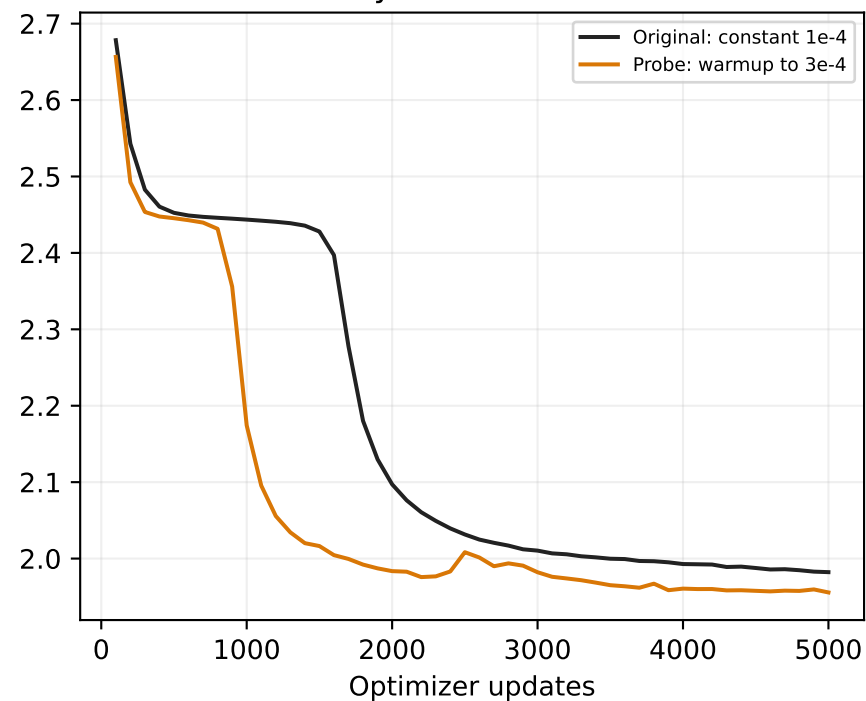
Fuzzy NextLat loss
