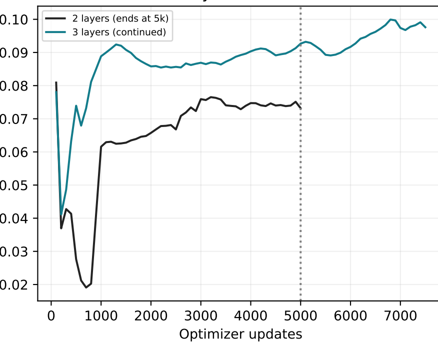
Fuzzy NextLat loss
