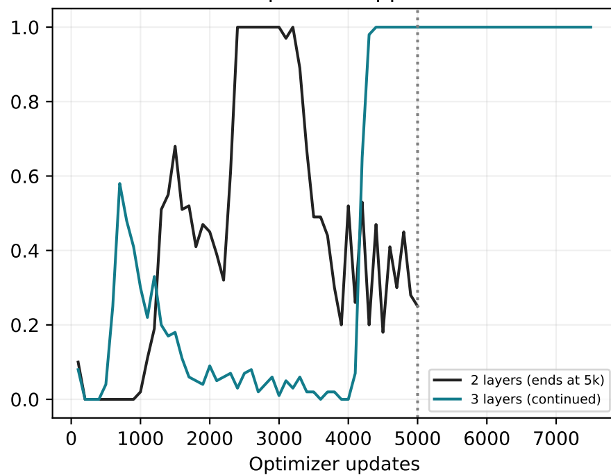
Fraction of updates clipped at norm1
