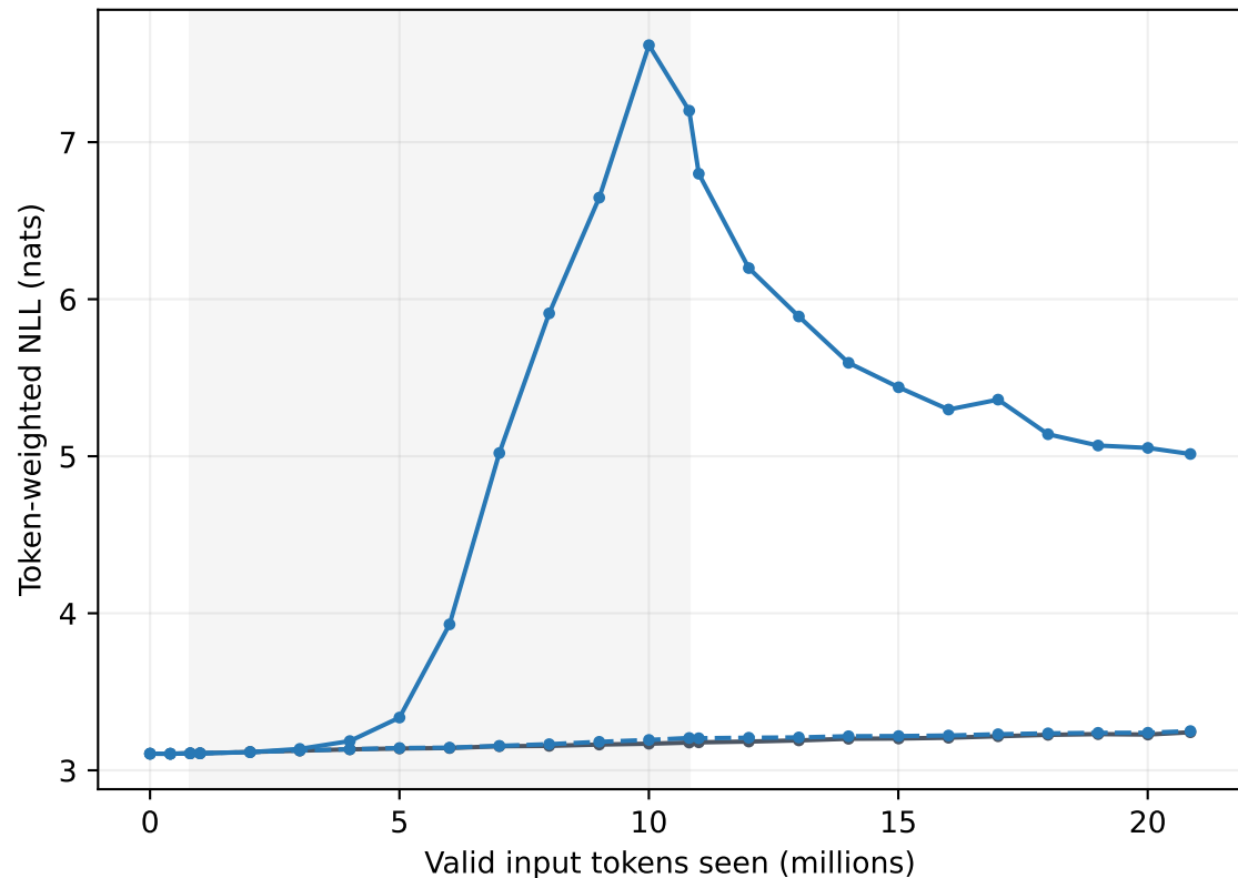
WikiText-2 language retention
