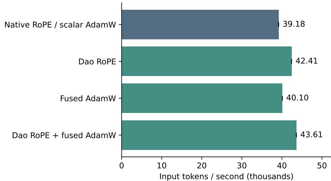
B64 / T512
