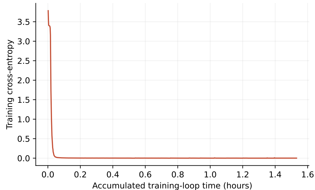
A5 RT · complete pilot + continuation history Nonoverlapping 100-update means; training time excludes evaluation/checkpointing/logging
