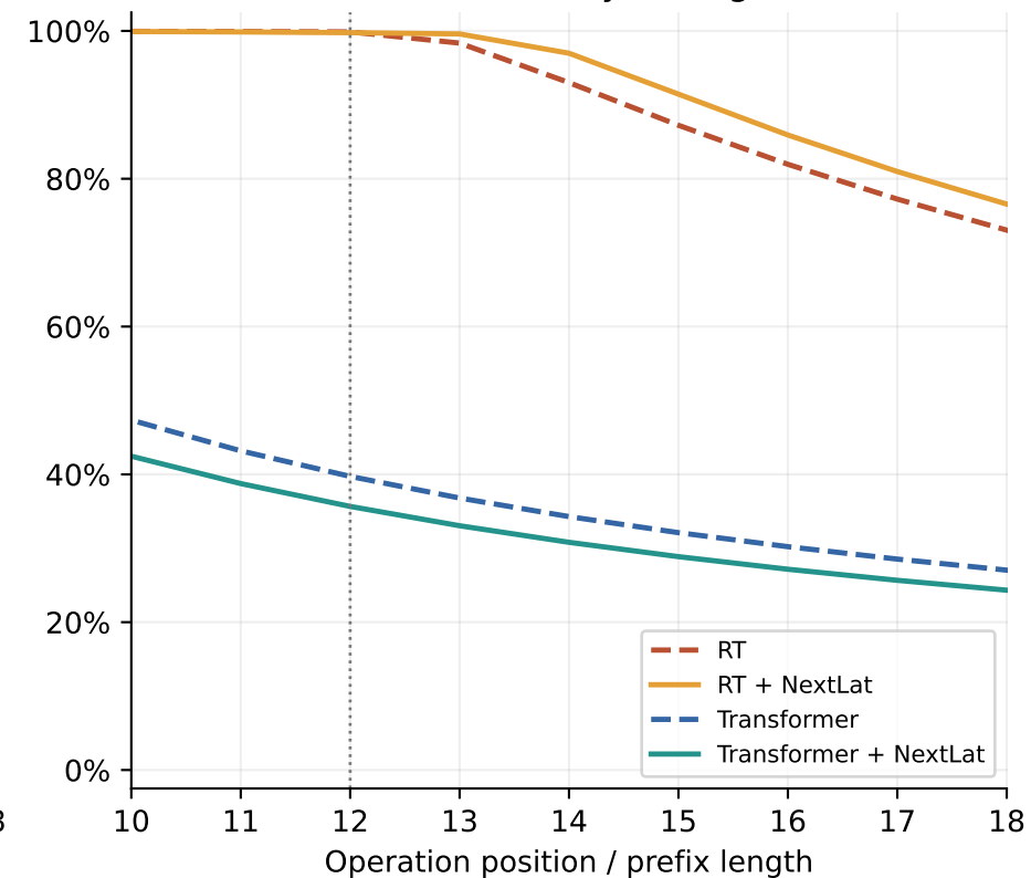
Mean token accuracy through t : M(t)
